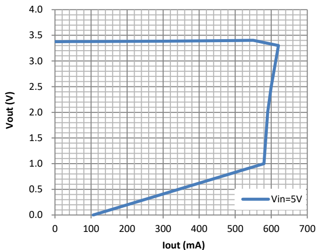
Current limit
